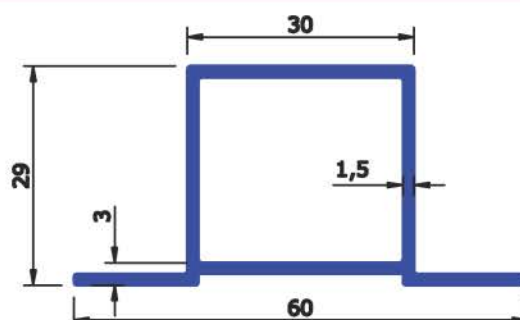
SEC No : 3971 WEIGHT Kg/Mtr 0.574
