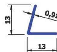
SEC No : 3921 WEIGHT Kg/Mtr 0.062
