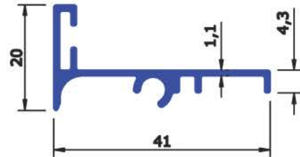
SEC No : 4059 WEIGHT Kg/Mtr 1.000 - 1.100
