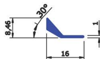
SEC No : 3922 WEIGHT Kg/Mtr 0.089
