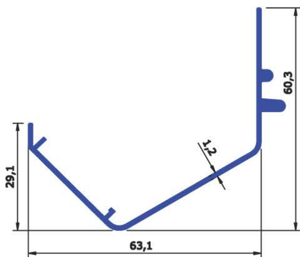
SEC No : 3918 WEIGHT Kg/Mtr 0.489
