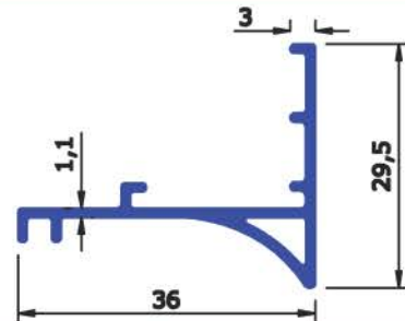
SEC No : 4063 WEIGHT Kg/Mtr 1.030 - 1.100
