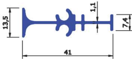
SEC No : 4060 WEIGHT Kg/Mtr 1.150 - 1.250
