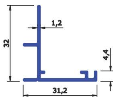
SEC No : 3925 WEIGHT Kg/Mtr 0.253
