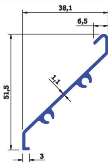
SEC No : 3923 WEIGHT Kg/Mtr 0.291
