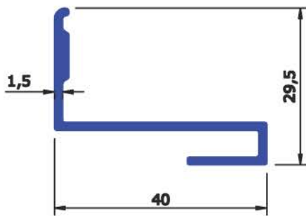
SEC No : 2876 WEIGHT Kg/Mtr 0.363
