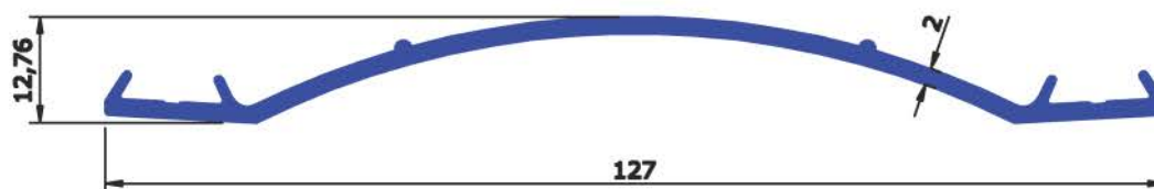
SECTION No : 2863 WEIGHT Kg/Mtr 0.737
