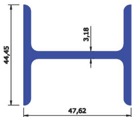
SEC No : 2856 WEIGHT Kg/Mtr 4.100 - 4.500
