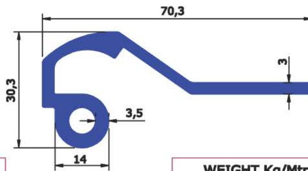
SECTION No : 2875 WEIGHT Kg/Mtr 1.051
