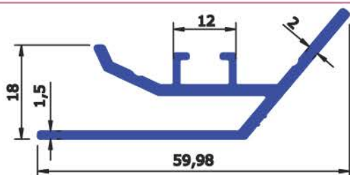
SEC No : 2882 WEIGHT Kg/Mtr 0.573
