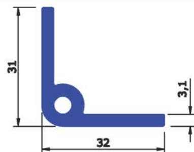
SEC No : 2880 WEIGHT Kg/Mtr 0.584
