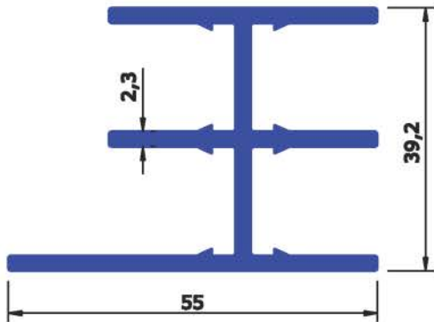
SEC No : 2873 WEIGHT Kg/Mtr 1.065
