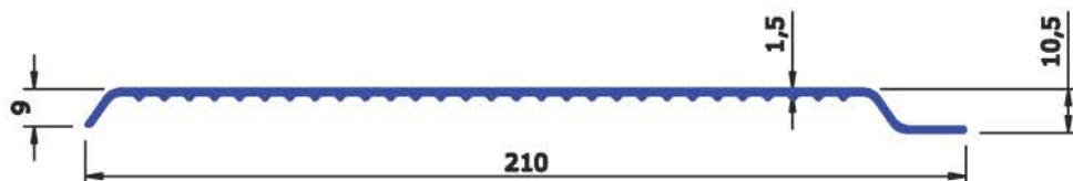
SECTION No : 2884 WEIGHT Kg/Mtr 1.038
