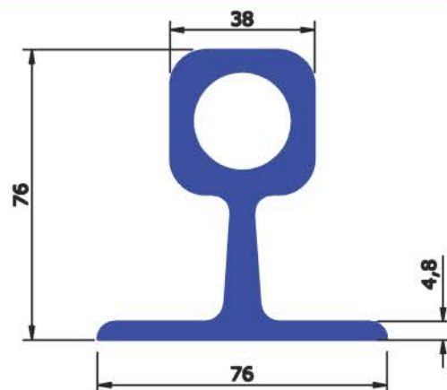
SEC No : 2860 WEIGHT Kg/Mtr 3.907
