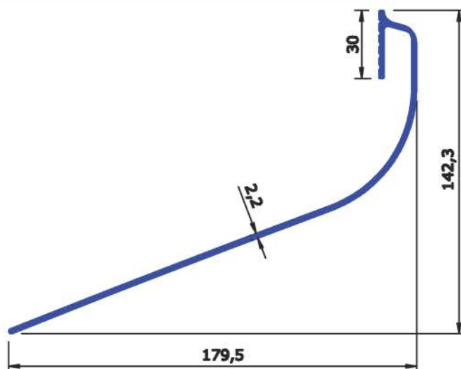
SECTION No : 2885 WEIGHT RANGE Kg/12' : 6.250 - 6.850
