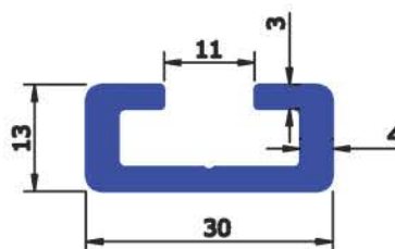
SEC No : 2883 WEIGHT Kg/Mtr 0.532
