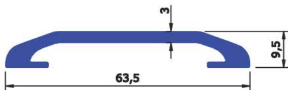
SEC No : 2865 WEIGHT Kg/Mtr 0.657
