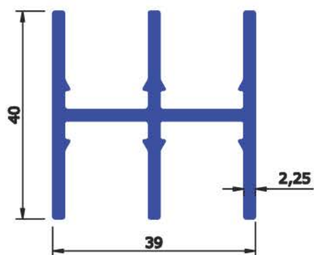
SEC No : 2870 WEIGHT Kg/Mtr 0.951
