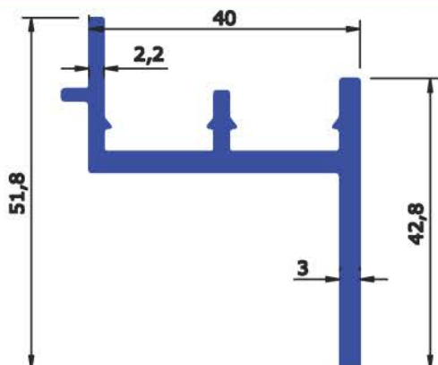
SEC No : 2878 WEIGHT Kg/Mtr 0.846
