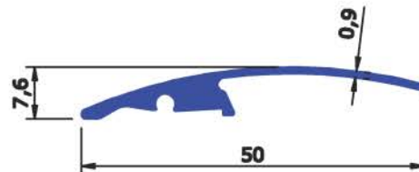
SEC No : 2869 WEIGHT Kg/Mtr 0.245
