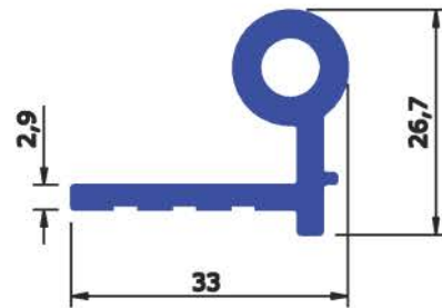
SEC No : 2874 WEIGHT Kg/Mtr 0.601
