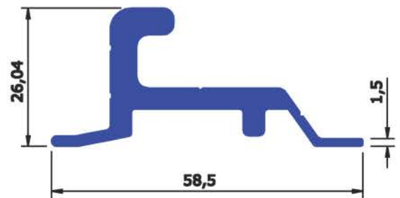
SEC No : 2877 WEIGHT Kg/Mtr 0.887
