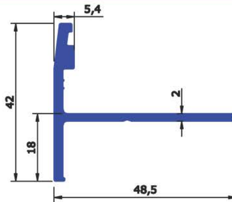
SEC No : 2881 WEIGHT Kg/Mtr 0.573
