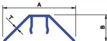
SEC No : 5205 WEIGHT Kg/Mtr 0.505
