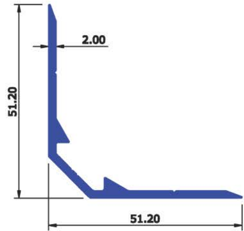
SEC No : 5210 WEIGHT Kg/Mtr 0.552
