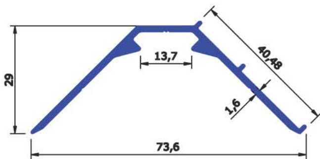
SEC No: 6618 WEIGHT KG/Mtr 0.486
