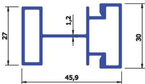
SEC No : 4248 WEIGHT Kg/Mtr 0.642
