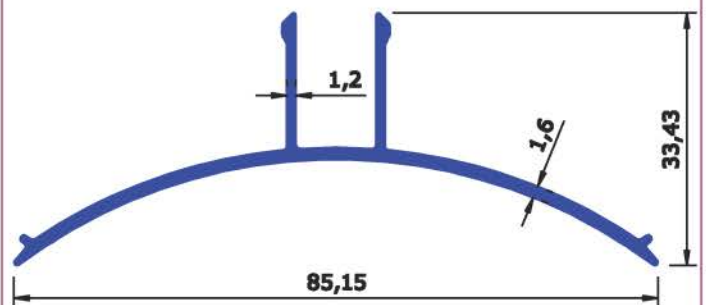
SEC No: 6619 WEIGHT KG/Mtr 0.518
