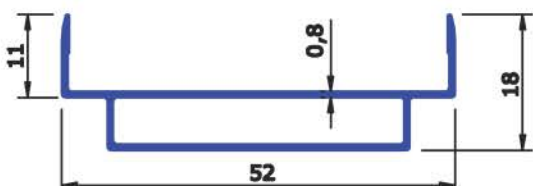
SEC No : 4252 WEIGHT Kg/Mtr 0.271
