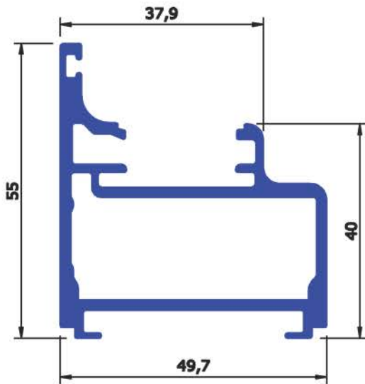
SEC No : 5242 WEIGHT Kg/Mtr 1.254
