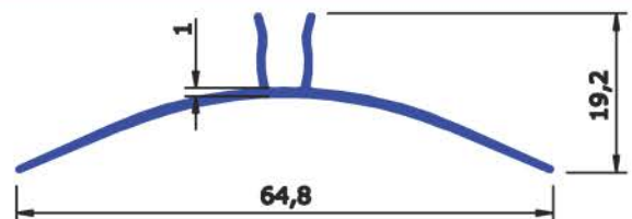
SEC No : 4250 WEIGHT Kg/Mtr 0.212
