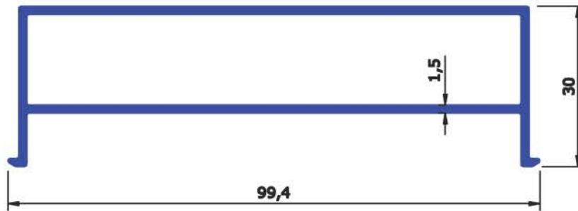
SECTION No : 6615 WEIGHT KG/Mtr 1.004
