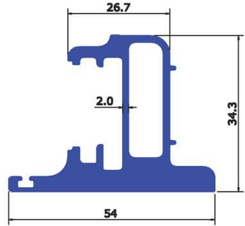
SEC No : 4381 WEIGHT Kg/Mtr 1.455
