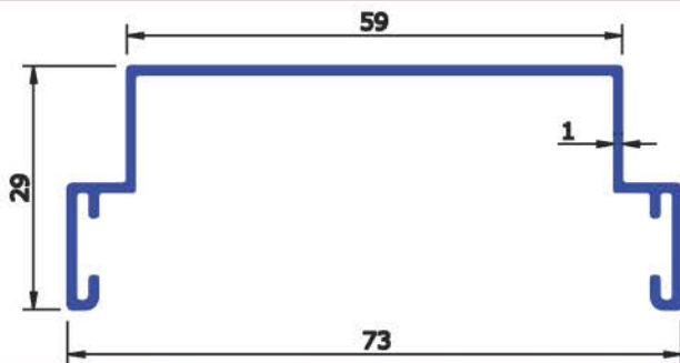
SEC No : 5296 WEIGHT Kg/Mtr 0.391
