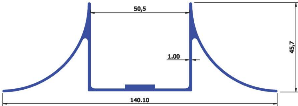
SECTION No : 5204 WEIGHT Kg/Mtr 0.928
