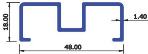
SEC No : 4241 WEIGHT Kg/Mtr 0.419
