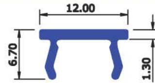
SEC No : 4243 WEIGHT Kg/Mtr 0.054
