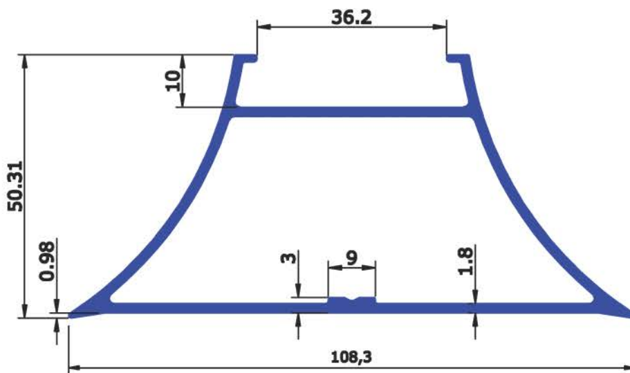
SECTION No : 4382 WEIGHT Kg/Mtr 1.343
