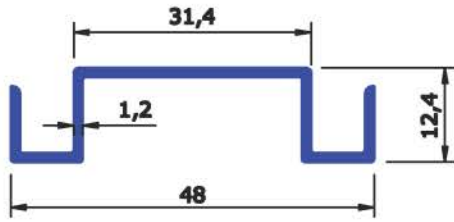
SEC No : 5293 WEIGHT Kg/Mtr 0.283
