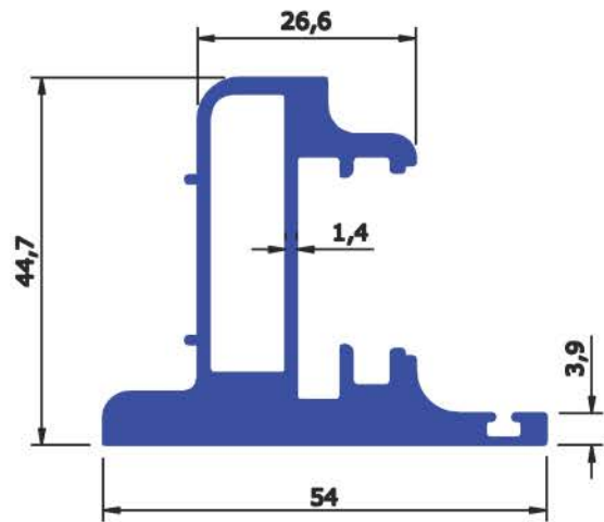
SEC No : 5243 WEIGHT Kg/Mtr 1.475
