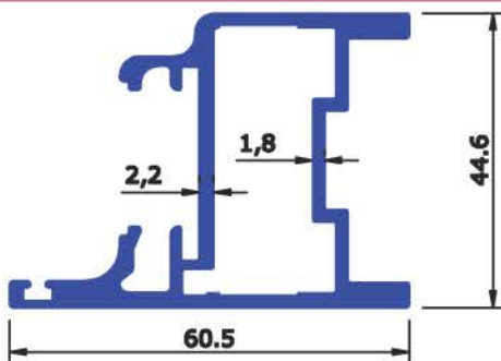
SEC No: 6603 WEIGHT KG/Mtr 0.838
