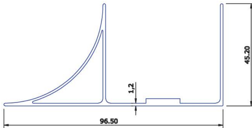
SECTION No : 5208 WEIGHT Kg/Mtr 0.839
