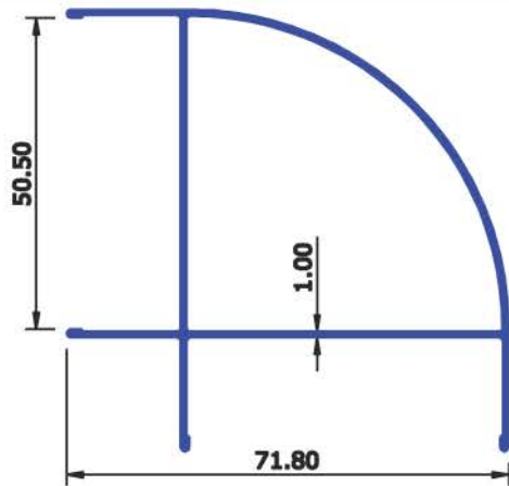
SEC No : 5201 WEIGHT Kg/Mtr 10.248
