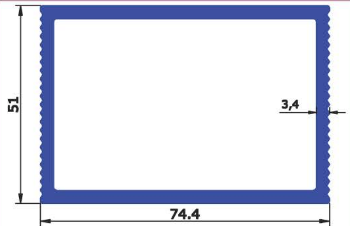
SEC No : 6602 WEIGHT Kg/Mtr 2.099
