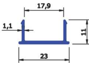
SEC No : 5244 WEIGHT Kg/Mtr 0.141
