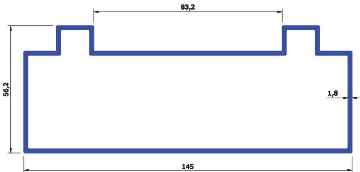
SECTION No : 5241 WEIGHT Kg/Mtr 2.029
