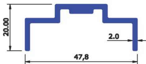
SEC No : 5205 WEIGHT Kg/Mtr 0.505
