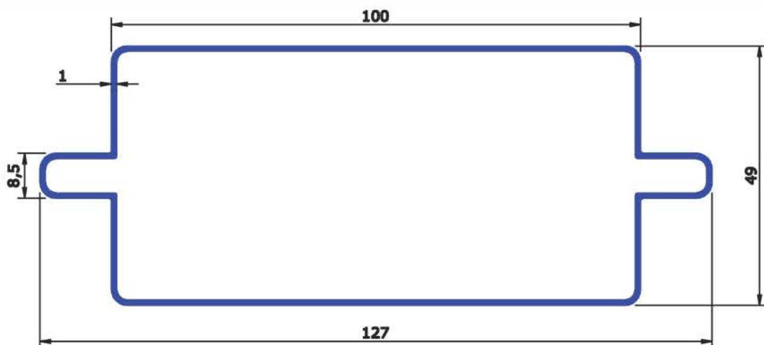
SECTION No : 4251 WEIGHT Kg/Mtr 0.916
