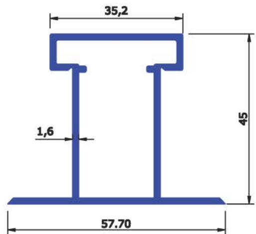
SEC No : 4246 WEIGHT Kg/Mtr 0.820
