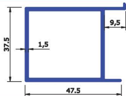
SEC No: 4254 WEIGHT KG/Mtr 0.574
