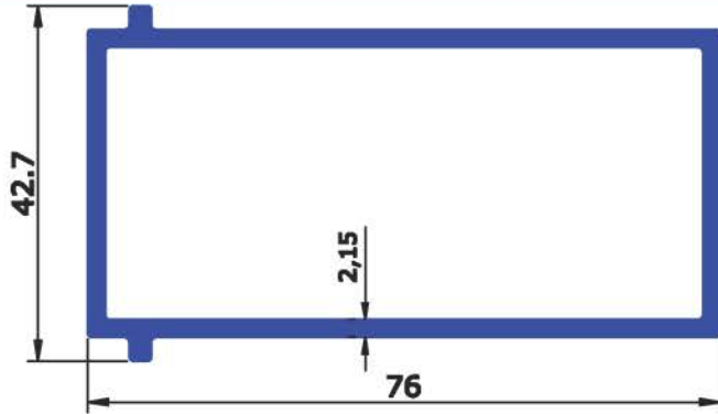
SEC No : 5296 WEIGHT Kg/Mtr 0.391
