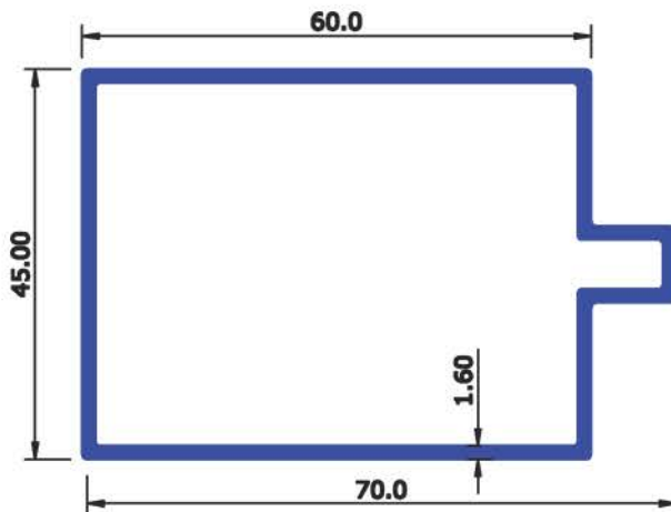
SEC No : 4242 WEIGHT Kg/Mtr 0.993
