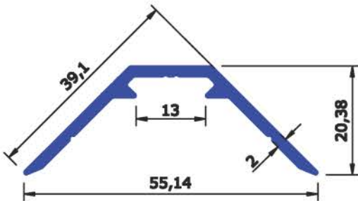
SEC No: 6616 WEIGHT KG/Mtr 0.397
