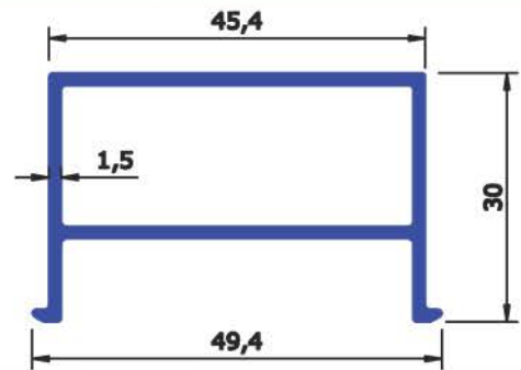
SEC No: 6614 WEIGHT KG/Mtr 0.599
