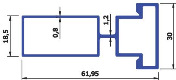
SEC No: 4255 WEIGHT KG/Mtr 0.594
