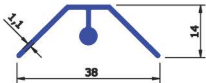
SEC No : 4249 WEIGHT Kg/Mtr 0.202
