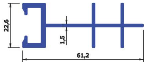
SEC No : 5245 WEIGHT Kg/Mtr 0.658
