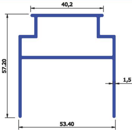
SEC No : 5207 WEIGHT Kg/Mtr 0.886
