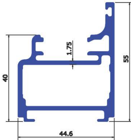
SEC No : 4380 WEIGHT Kg/Mtr 1.145
