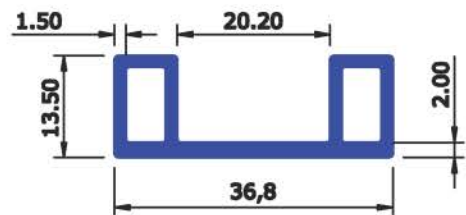
SEC No : 5217 WEIGHT Kg/Mtr 0.427
