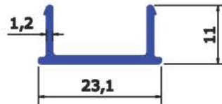
SECTION No : 4260 WEIGHT Kg/Mtr 0.153
