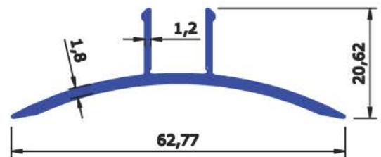
SEC No: 6617 WEIGHT KG/Mtr 0.382
