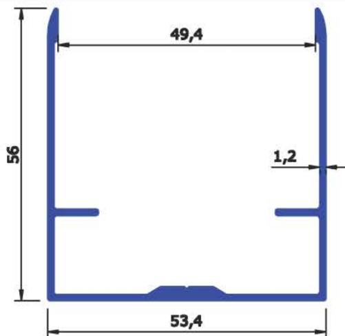
SEC No : 4245 WEIGHT Kg/Mtr 0.653
