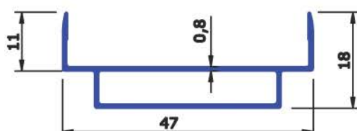
SEC No : 4253 WEIGHT Kg/Mtr 0.250
