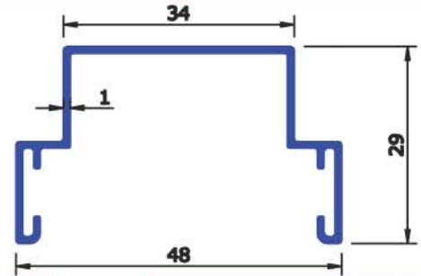
SEC No : 5295 WEIGHT Kg/Mtr 0.324
