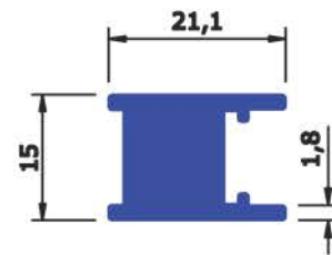
SEC No : 6606 WEIGHT Kg/Mtr 0.585
