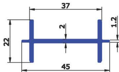
SEC No : 6605 WEIGHT Kg/Mtr 0.438
