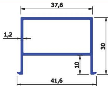
SEC No : 4247 WEIGHT Kg/Mtr 0.421
