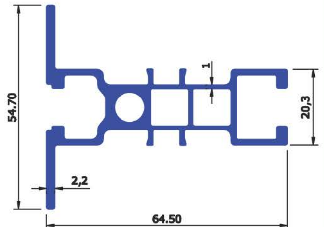
SEC No : 4244 WEIGHT Kg/Mtr 1.160
