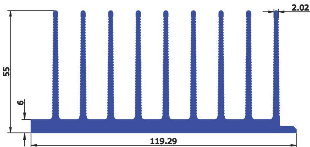
SECTION No : 3094 WEIGHT Kg/Mtr 4.394
