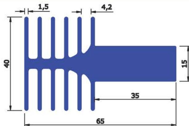
SEC No : 3097 WEIGHT Kg/Mtr 2.718
