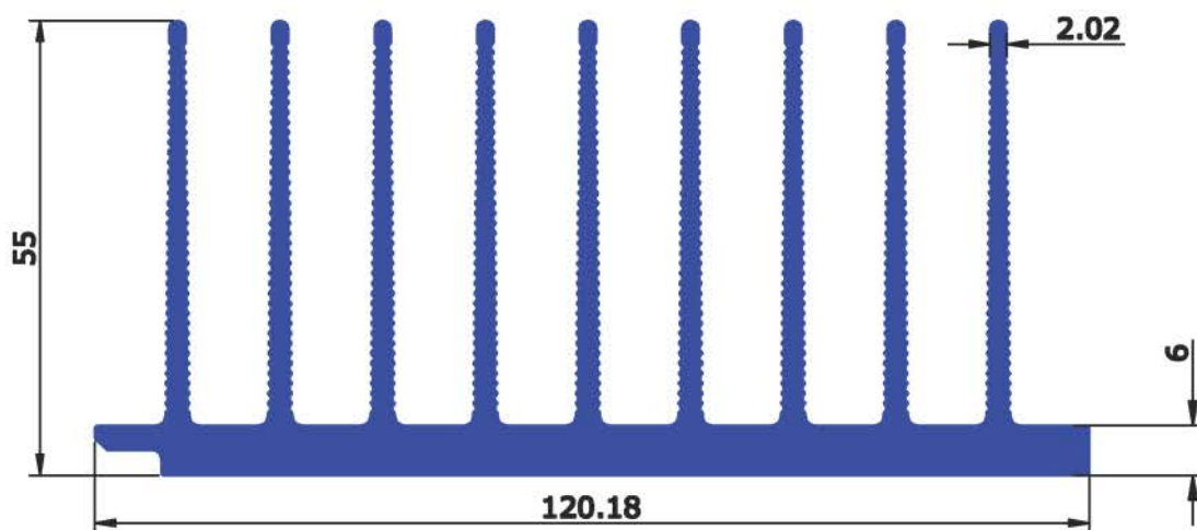
SECTION No : 3095 WEIGHT Kg/Mtr 4.407
