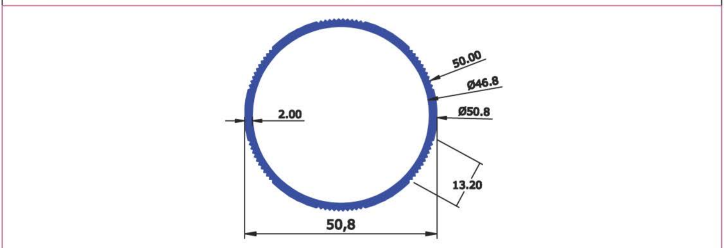
SECTION No : 5028 WEIGHT KG/Mtr 0.737
