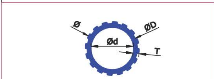
SEC No : 4889 WEIGHT Kg/Mtr 2.814
