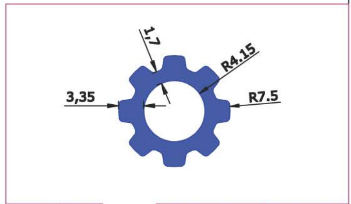
SEC No : 7922 WEIGHT Kg/Mtr 0.245
