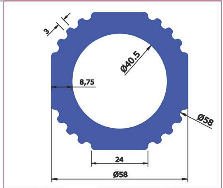
SEC No : 4890 WEIGHT Kg/Mtr 4.057
