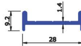
SEC No : 6331 WEIGHT Kg/Mtr 0.169
