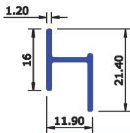
SEC No : 6121 WEIGHT Kg/Mtr 0.130
