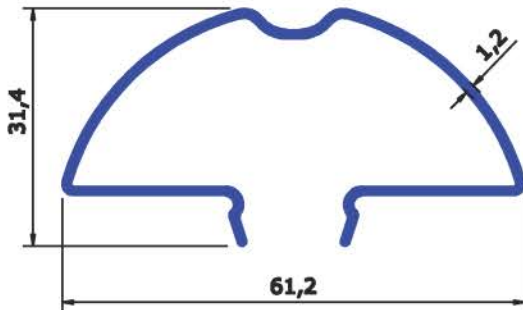
SEC No : 5194 WEIGHT Kg/Mtr 0.464
