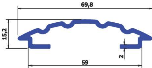
SEC No : 5195 WEIGHT Kg/Mtr 0.608
