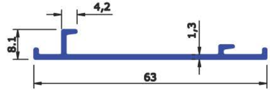
SEC No : 6441 WEIGHT Kg/Mtr 0.281
