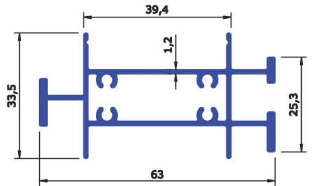
SEC No : 6456 WEIGHT Kg/Mtr 0.824
