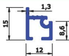
SEC No : 5270 WEIGHT Kg/Mtr 0.157
