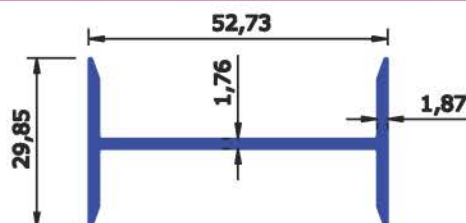
SEC No : 6568 WEIGHT Kg/Mtr 0.573
