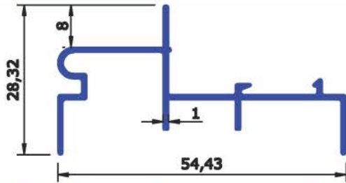
SEC No : 6591 WEIGHT Kg/Mtr 0.343
