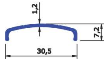
SEC No : 5184 WEIGHT Kg/Mtr 0.123
