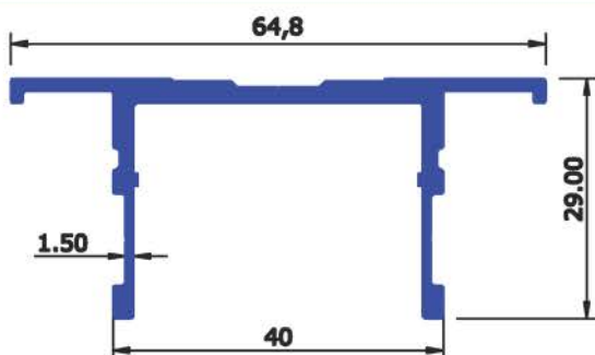
SEC No : 6409 WEIGHT Kg/Mtr 0.650
