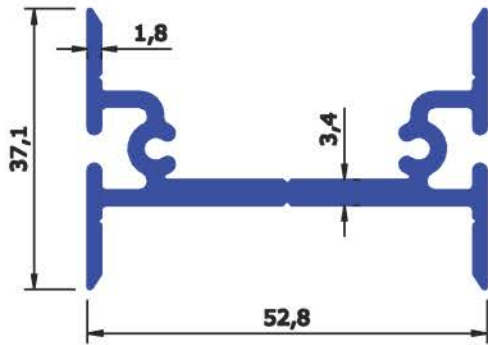
SEC No : 3053 WEIGHT Kg/Mtr 0.955
