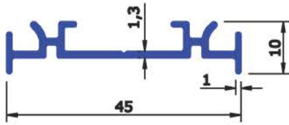
SEC No : 6327 WEIGHT Kg/Mtr 0.280
