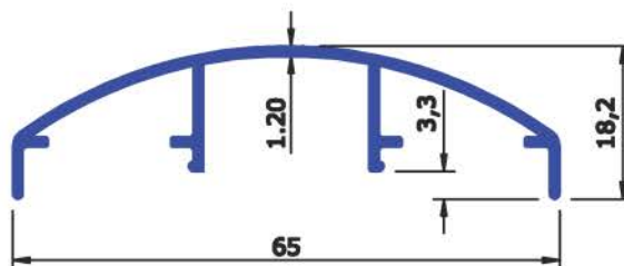
SEC No : 6414 WEIGHT Kg/Mtr 0.385
