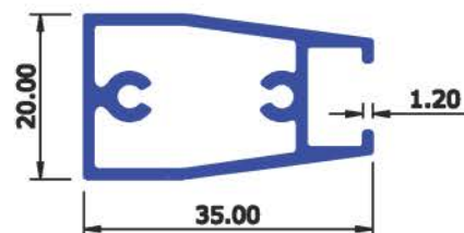
SEC No : 5057 WEIGHT Kg/Mtr 0.440
