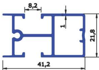
SEC No: 6758 WEIGHT KG/Mtr 0.441
