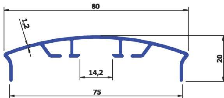
SECTION No : 5187 WEIGHT Kg/Mtr 0.481
