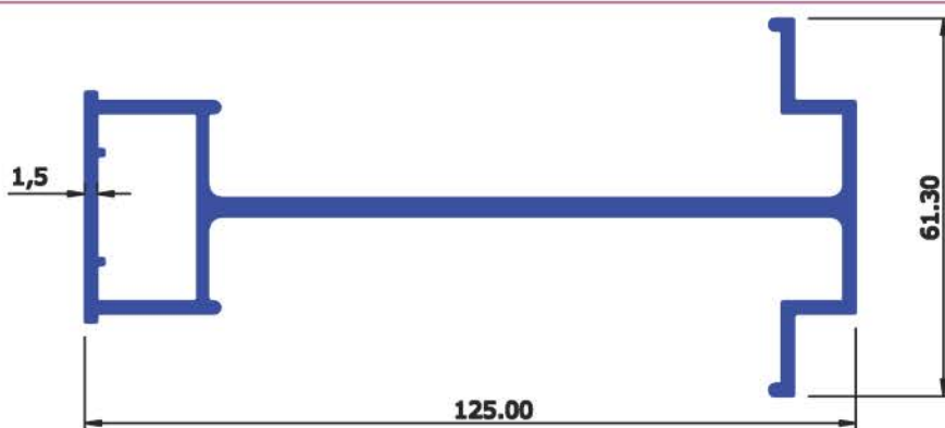
SECTION No : 6403 WEIGHT Kg/Mtr 1.052
