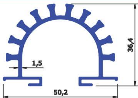
SEC No : 6546 WEIGHT Kg/Mtr 0.800
