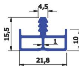
SEC No: 6759 WEIGHT KG/Mtr 0.240
