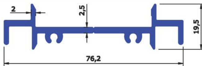
SECTION No : 4562 WEIGHT Kg/Mtr 0.841
