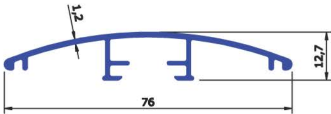
SEC No : 5054 WEIGHT Kg/Mtr 0.401
