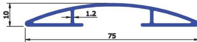
SECTION No : 6316 WEIGHT Kg/Mtr 0.437
