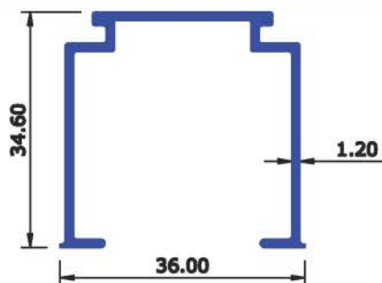
SEC No : 6401 WEIGHT Kg/Mtr 0.380
