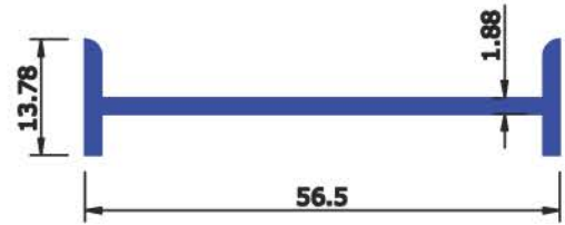
SEC No : 6592 WEIGHT Kg/Mtr 0.410
