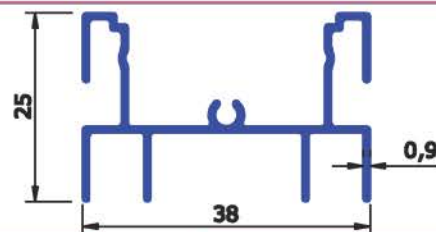
SEC No : 6148 WEIGHT Kg/Mtr 0.337
