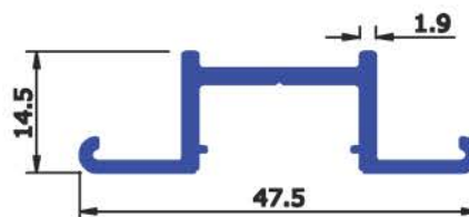
SEC No : 6321 WEIGHT Kg/Mtr 0.361
