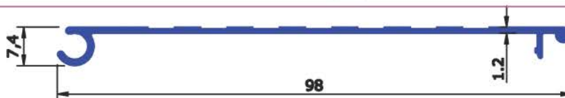
SECTION No : 6324 WEIGHT Kg/Mtr 0.346
