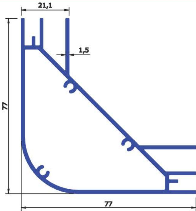
SEC No : 5156 WEIGHT Kg/Mtr 1.311
