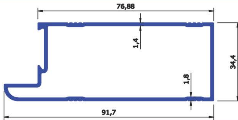
SECTION No : 6593 WEIGHT Kg/Mtr 0.969
