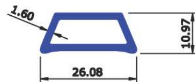
SEC No : 5162 WEIGHT Kg/Mtr 0.245
