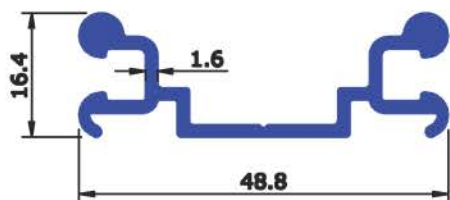
SEC No : 6322 WEIGHT Kg/Mtr 0.523
