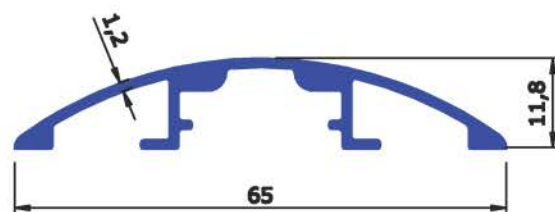
SEC No : 6411 WEIGHT Kg/Mtr 0.442
