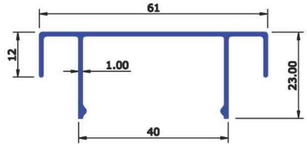
SEC No : 6112 WEIGHT Kg/Mtr 0.352
