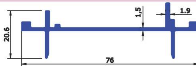
SECTION No : 7144 WEIGHT Kg/Mtr 0.574
