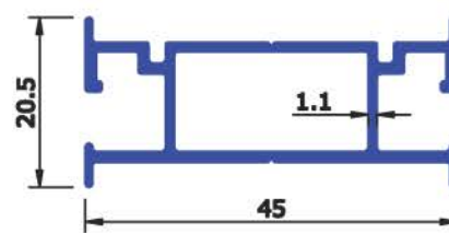
SEC No : 6326 WEIGHT Kg/Mtr 0.456
