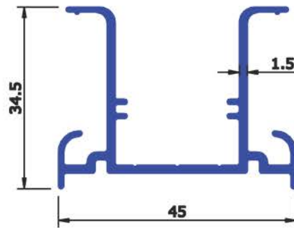
SECTION No : 6328 WEIGHT Kg/Mtr 0.563
