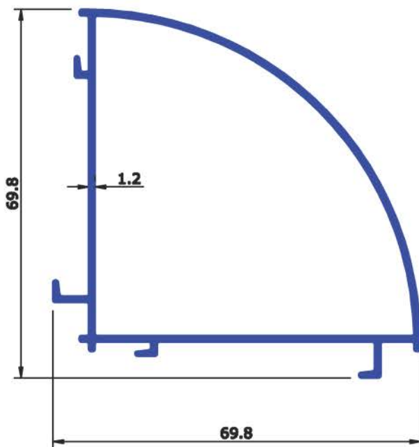
SEC No : 6442 WEIGHT Kg/Mtr 0.834
