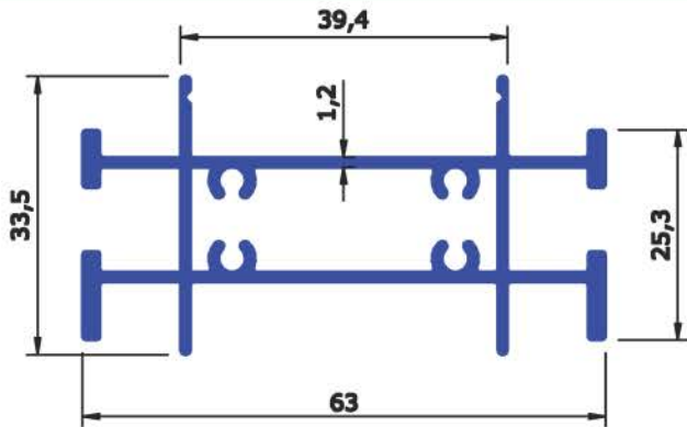
SEC No : 6455 WEIGHT Kg/Mtr 0.884
