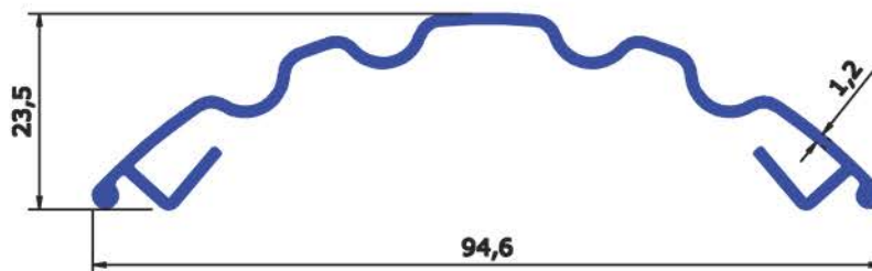
SECTION No : 5196 WEIGHT Kg/Mtr 0.504
