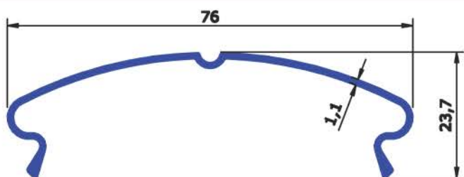
SEC No: 6756 WEIGHT KG/Mtr 0.355
