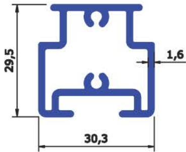
SEC No : 5192 WEIGHT Kg/Mtr 0.655
