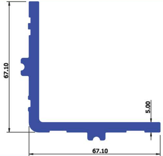
SEC No : 6502 WEIGHT Kg/Mtr 1.832
