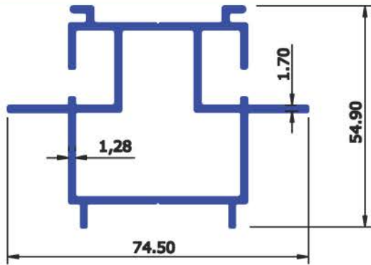
SEC No : 5052 WEIGHT Kg/Mtr 1.256
