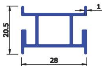
SEC No : 6325 WEIGHT Kg/Mtr 0.339
