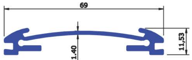
SEC No : 5056 WEIGHT Kg/Mtr 0.616
