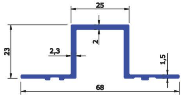
SEC No : 6506 WEIGHT Kg/Mtr 0.563
