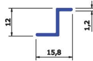
SEC No : 5193 WEIGHT Kg/Mtr 0.086
