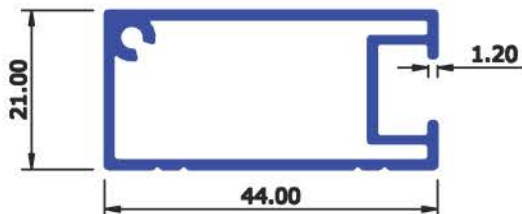
SEC No : 5058 WEIGHT Kg/Mtr 0.495
