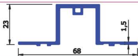
SEC No : 6562 WEIGHT Kg/Mtr 0.601
