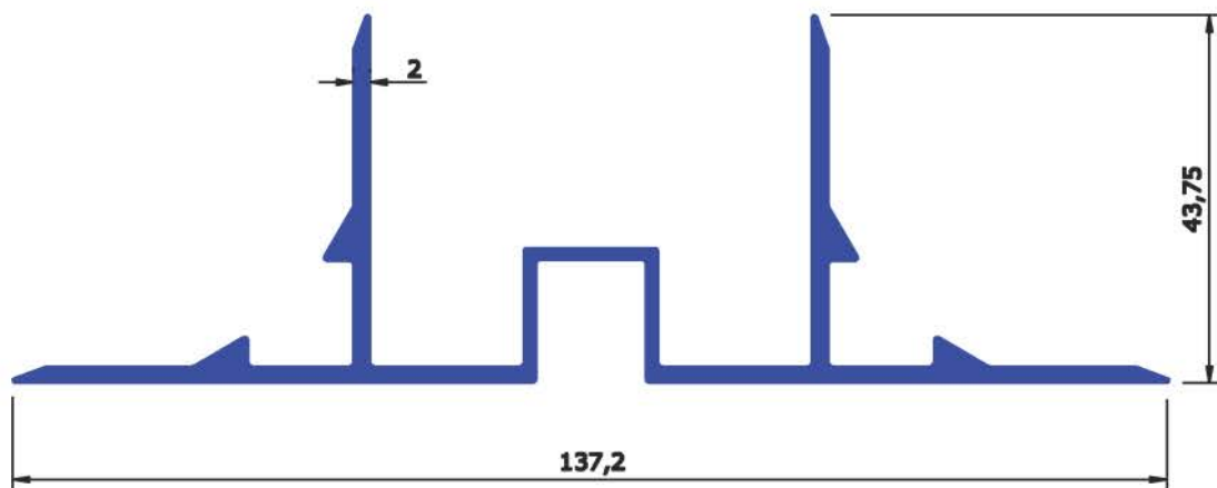
SECTION No : 6536 WEIGHT Kg/Mtr 1.3866
