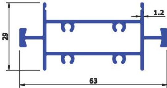
SEC No : 6446 WEIGHT Kg/Mtr 0.707
