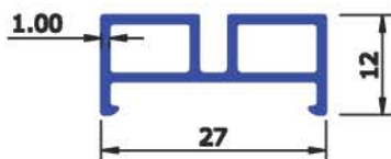
SEC No : 5161 WEIGHT Kg/Mtr 0.227
