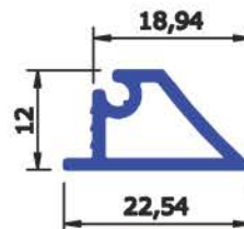
SEC No : 5269 WEIGHT Kg/Mtr 0.191
