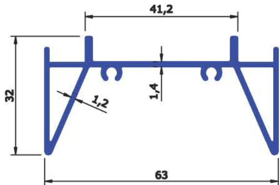
SEC No : 6460 WEIGHT Kg/Mtr 0.683
