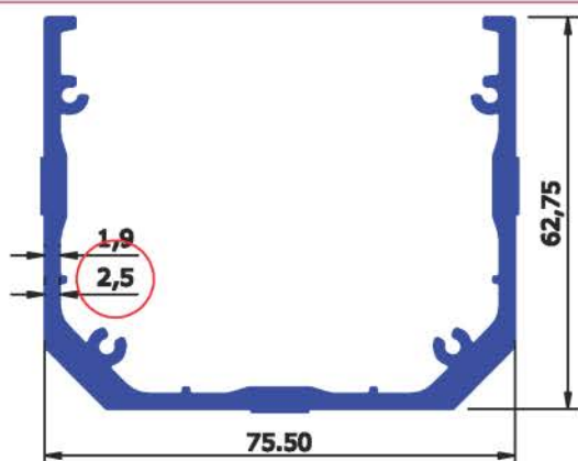
SEC No : 6151 WEIGHT Kg/Mtr 1.748
