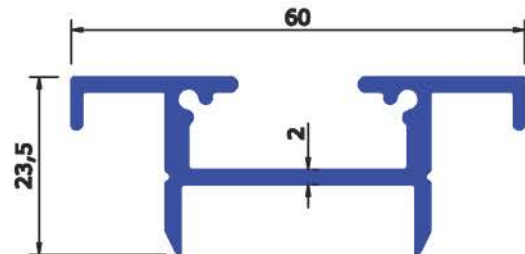
SEC No : 5198 WEIGHT Kg/Mtr 0.709
