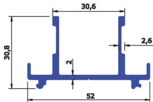
SEC No : 6124 WEIGHT Kg/Mtr 0.623
