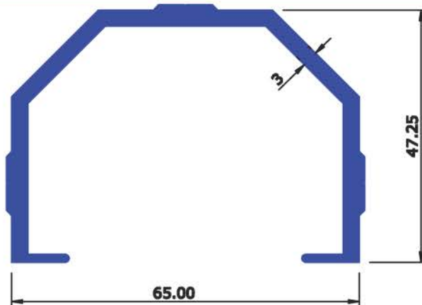
SEC No : 6406 WEIGHT Kg/Mtr 1.247
