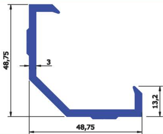
SEC No : 6405 WEIGHT Kg/Mtr 0.898
