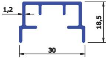
SEC No : 5181 WEIGHT Kg/Mtr 0.268
