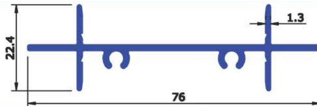
SECTION No : 7143 WEIGHT Kg/Mtr 0.520
