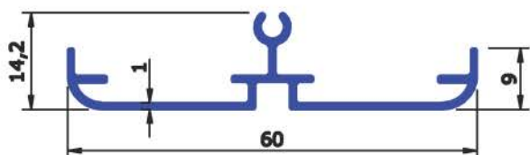
SEC No: 6751 WEIGHT KG/Mtr 0.300
