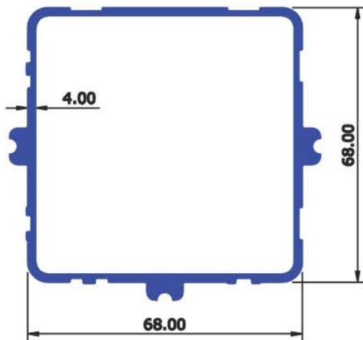
SEC No : 6504 WEIGHT Kg/Mtr 2.732
