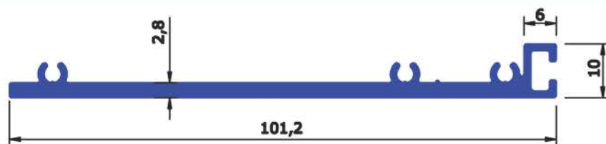
SECTION No : 5271 WEIGHT Kg/Mtr 0.878
