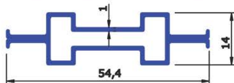
SEC No : 6561 WEIGHT Kg/Mtr 0.413
