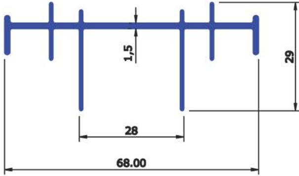
SEC No : 6501 WEIGHT Kg/Mtr 0.558
