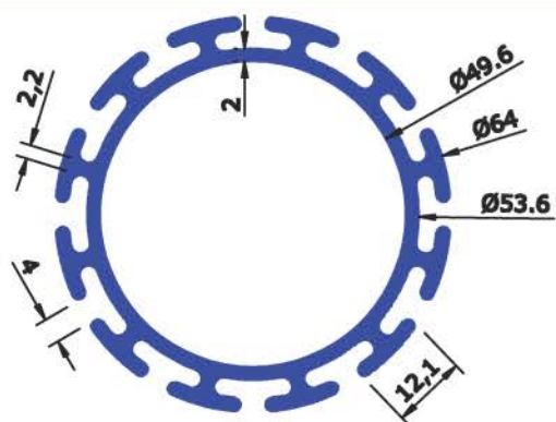
SEC No : 5266 WEIGHT Kg/Mtr 1.967
