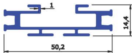
SEC No : 6547 WEIGHT Kg/Mtr 0.482
