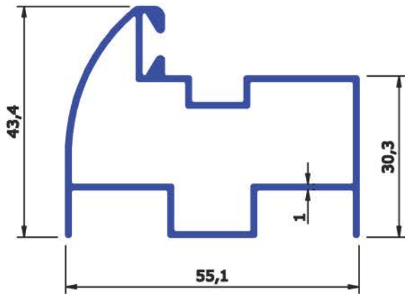
SEC No : 6531 WEIGHT Kg/Mtr 0.630
