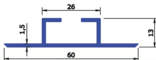
SEC No: 5300 WEIGHT KG/Mtr 0.386
