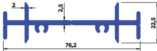
SECTION No : 4561 WEIGHT Kg/Mtr 0.939
