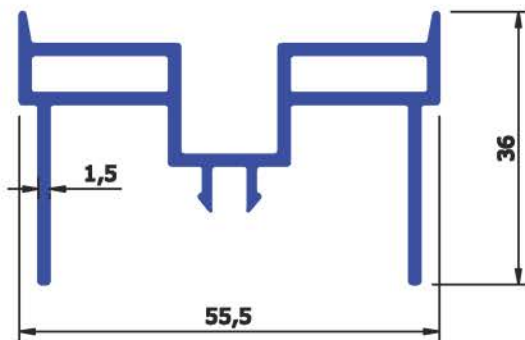
SEC No : 6534 WEIGHT Kg/Mtr 0.792
