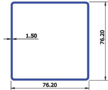
SEC No : 5053 WEIGHT Kg/Mtr 1.202
