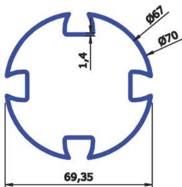
SEC No : 6318 WEIGHT Kg/Mtr 1.188
