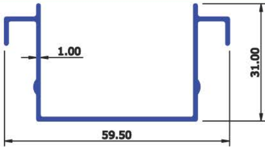
SEC No : 6111 WEIGHT Kg/Mtr 0.368
