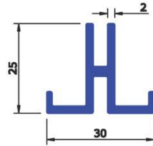
SEC No : 5158 WEIGHT Kg/Mtr 0.437
