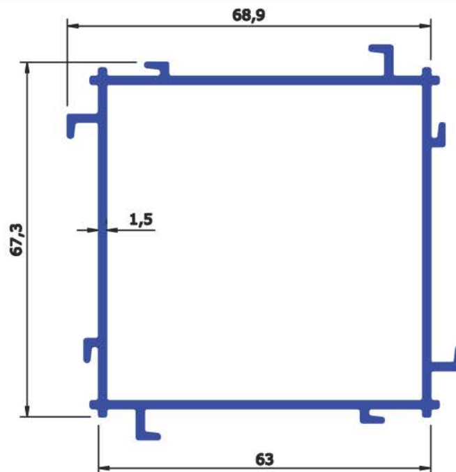
SECTION No : 6451 WEIGHT Kg/Mtr 1.265
