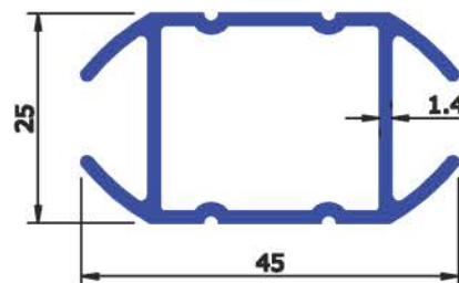
SEC No : 6319 WEIGHT Kg/Mtr 0.546
