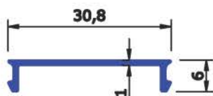
SEC No: 6755 WEIGHT KG/Mtr 0.115
