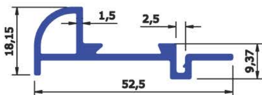
SEC No : 6564 WEIGHT Kg/Mtr 0.460
