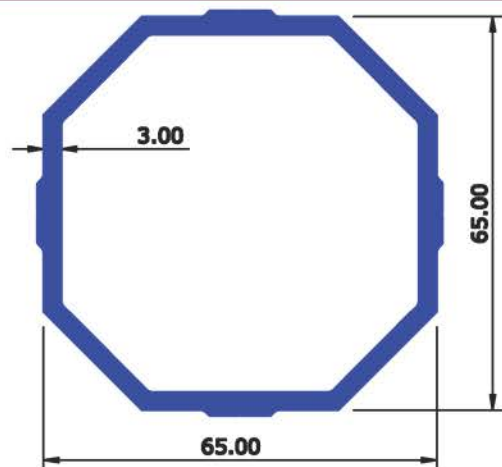
SEC No : 6407 WEIGHT Kg/Mtr 1.844
