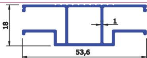
SEC No : 6550 WEIGHT Kg/Mtr 0.421
