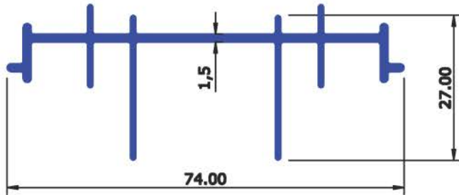
SEC No : 6503 WEIGHT Kg/Mtr 0.585
