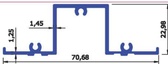
SECTION No : 6565 WEIGHT Kg/Mtr 0.522
