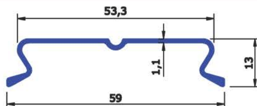
SEC No: 6757 WEIGHT KG/Mtr 0.269
