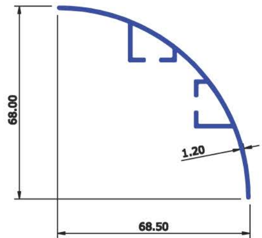
SEC No : 6505 WEIGHT Kg/Mtr 0.478
