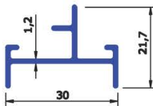
SECTION No : 5059 WEIGHT Kg/Mtr 0.242
