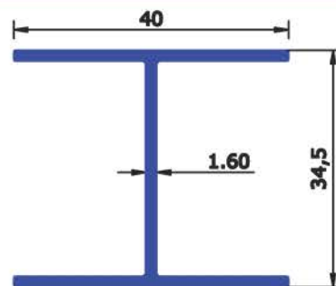
SEC No : 6402 WEIGHT Kg/Mtr 0.480
