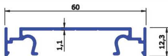
SEC No: 6753 WEIGHT KG/Mtr 0.358
