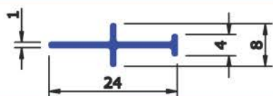
SEC No : 6548 WEIGHT Kg/Mtr 0.091
