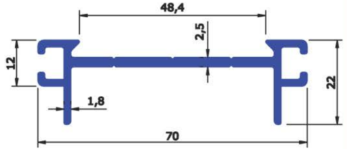
SEC No : 3052 WEIGHT Kg/Mtr 0.747
