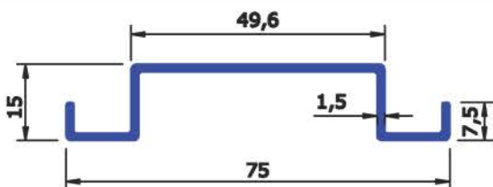
SEC No : 5264 WEIGHT Kg/Mtr 0.450
