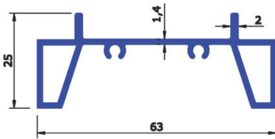
SEC No : 6448 WEIGHT Kg/Mtr 0.652
