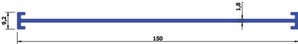
SECTION No : 5157 WEIGHT Kg/Mtr 0.839
