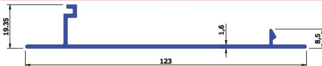
SECTION No : 6413 WEIGHT Kg/Mtr 0.667
