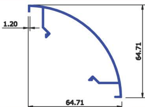
SEC No : 6412 WEIGHT Kg/Mtr 0.500
