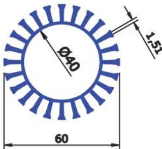
SEC No : 5185 WEIGHT Kg/Mtr 1.523
