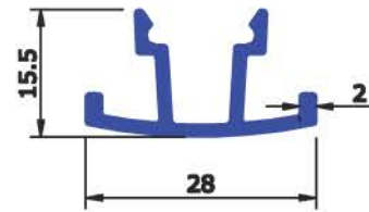
SEC No : 6329 WEIGHT Kg/Mtr 0.267
