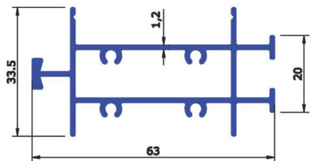
SEC No : 6445 WEIGHT Kg/Mtr 0.756
