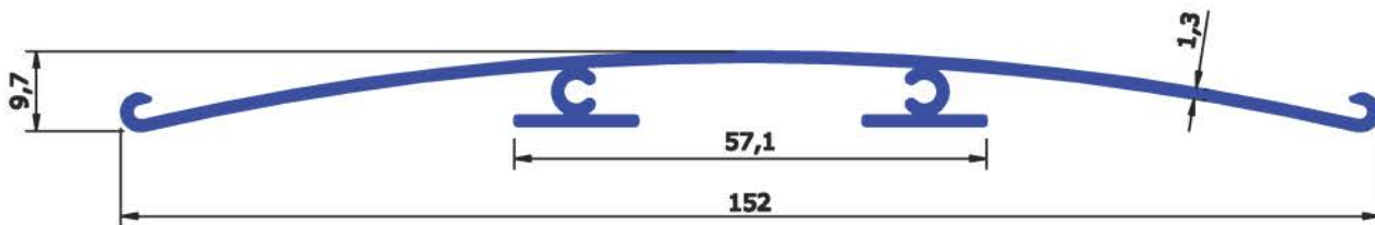
SECTION No : 5159 WEIGHT Kg/Mtr 0.754
