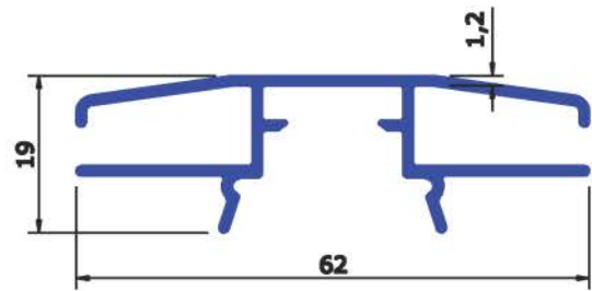
SEC No : 5197 WEIGHT Kg/Mtr 0.491
