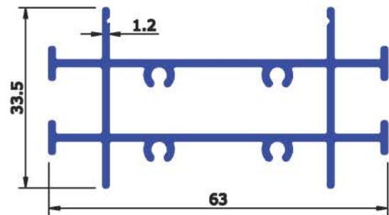
SEC No : 6449 WEIGHT Kg/Mtr 0.776
