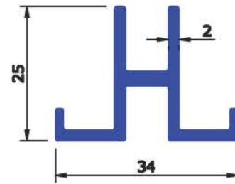
SEC No : 5160 WEIGHT Kg/Mtr 0.480
