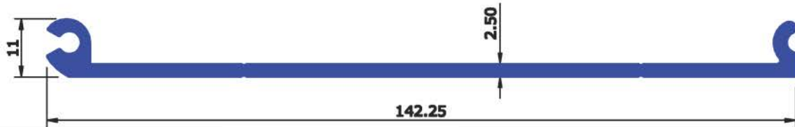
SECTION No : 5055 WEIGHT Kg/Mtr 1.115
