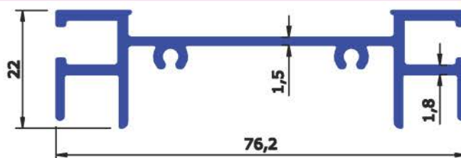
SECTION No : 7259 WEIGHT Kg/Mtr 0.796
