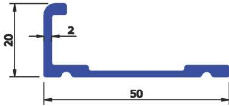
SEC No : 6415 WEIGHT Kg/Mtr 0.408
