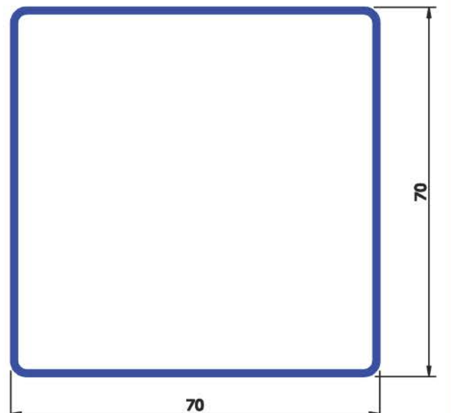
SEC No : 3056 WEIGHT Kg/Mtr 0.914
