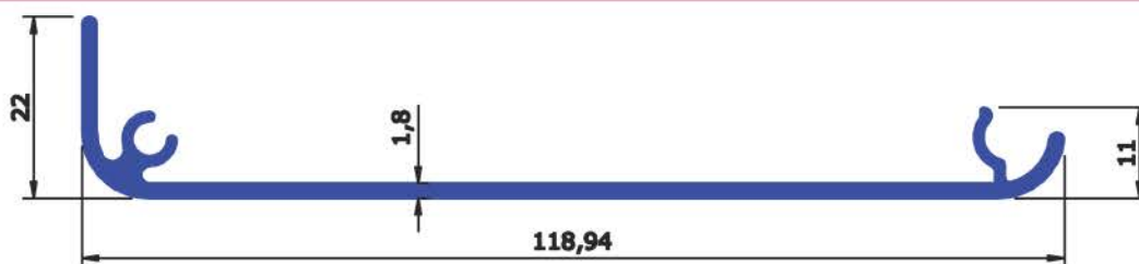
SECTION No : 6150 WEIGHT Kg/Mtr 0.777
