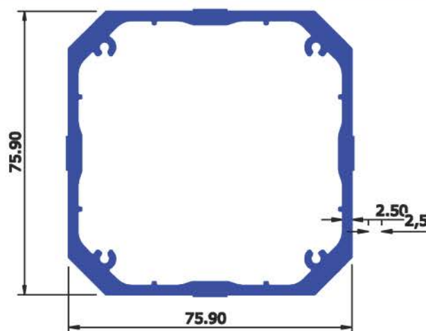
SECTION No : 6152 WEIGHT Kg/Mtr 2.568
