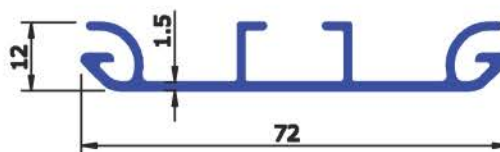
SEC No : 5272 WEIGHT Kg/Mtr 0.546
