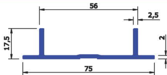
SEC No : 5265 WEIGHT Kg/Mtr 0.346
