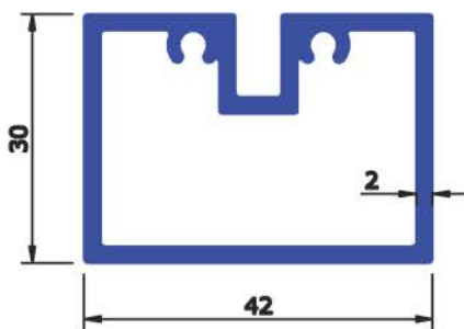
SEC No : 3049 WEIGHT Kg/Mtr 0.907
