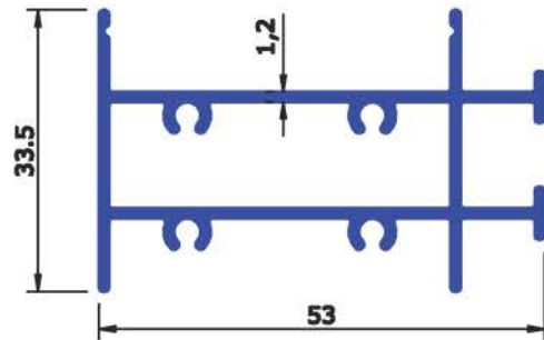
SEC No :- 6447 WEIGHT Kg/Mtr 0.679
